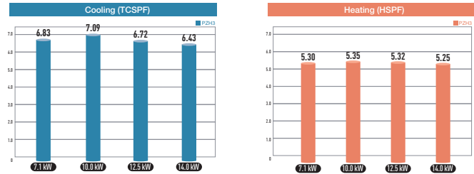
* The graph shows 4-WAY Cassette R32 Deluxe models values. * TCSPF/HSPF is based on Commercial (Average)
