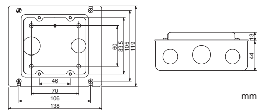
Switch Box
