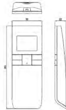
WIRELESS REMOTE CONTROLLER (CZ-RWS3)
