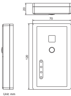
SEPARATE RECEIVER FOR WIRELESS REMOTE CONTROLLER (CZ-RWRC3)
