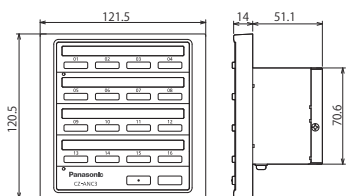
ON/OFF Controller
