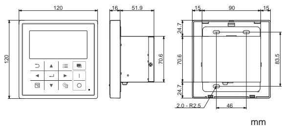
System Controller
